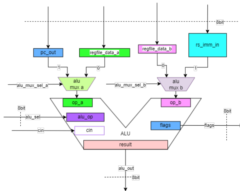
Figure 2: ALU
